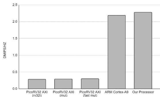
Figure 3 Dhrystone Benchmark Performance
