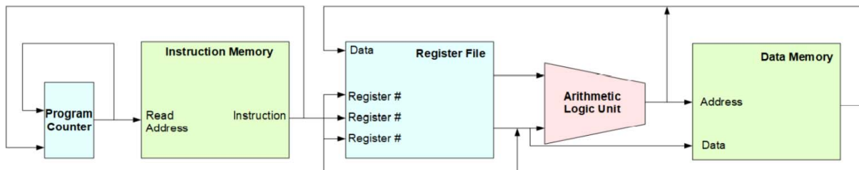
Figure 1 Processor Architecture
